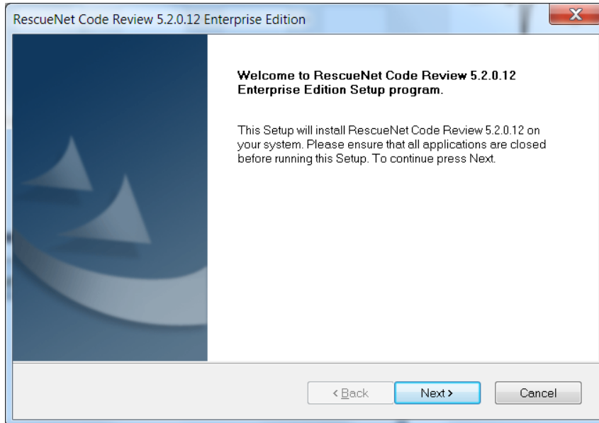
Figure 5 Welcome Screen
