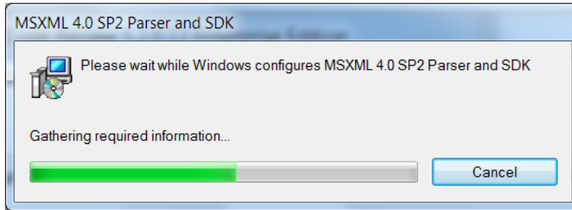
Figure 9 Install MSXML
